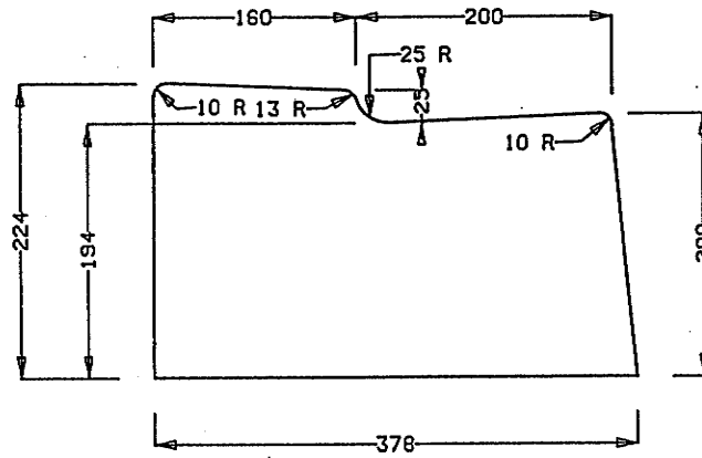
CURB AT DRIVEWAY CROSSING
