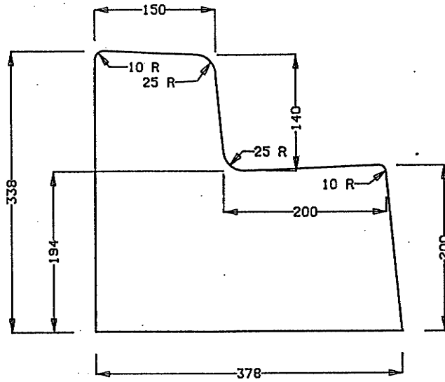
NON-MOUNTABLE CURB
